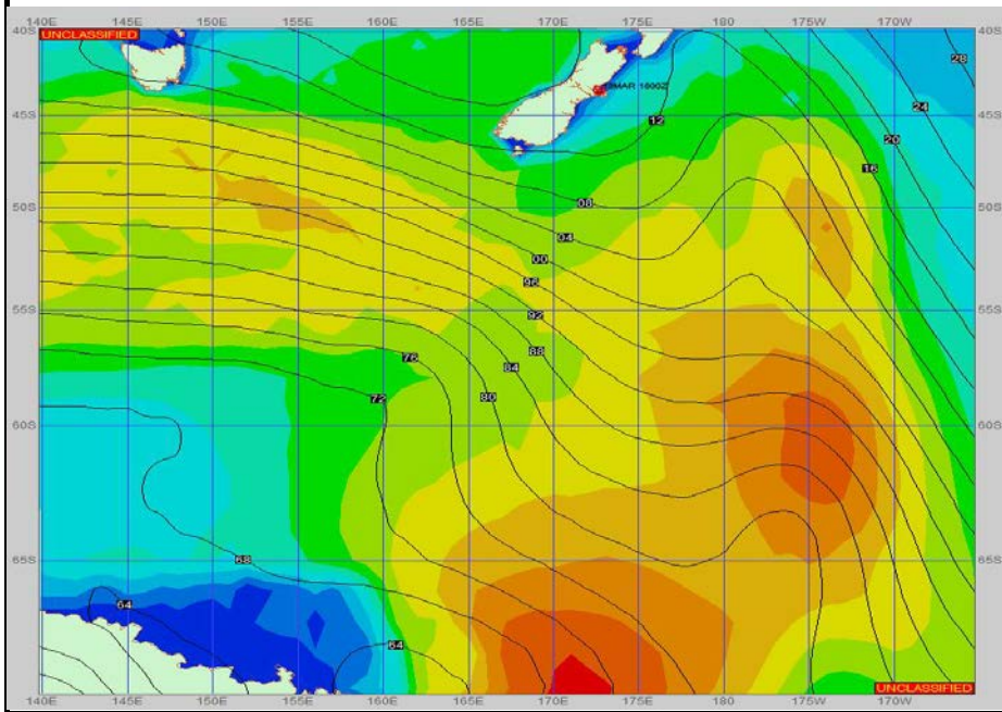
SURFACE ANALYSIS 17-Mar-2023 21Z
