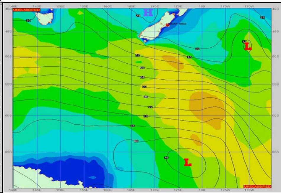
SURFACE FORECAST 18-Mar-2023 18Z
