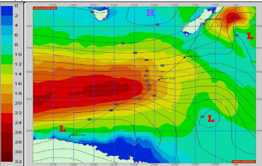
SURFACE FORECAST 22-Mar-2023 06Z
