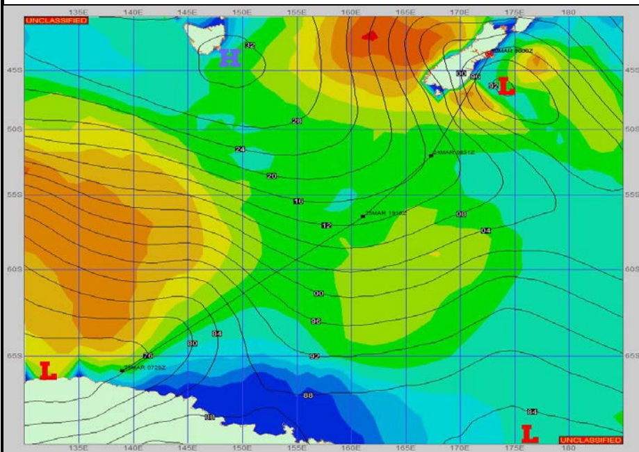
SURFACE ANALYSIS 20-Mar-2023 18Z
