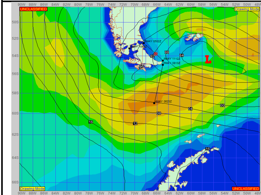
SURFACE ANALYSIS 5-May-2024 18Z
