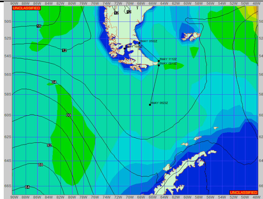
SURFACE FORECAST 7-May-2024 06Z
